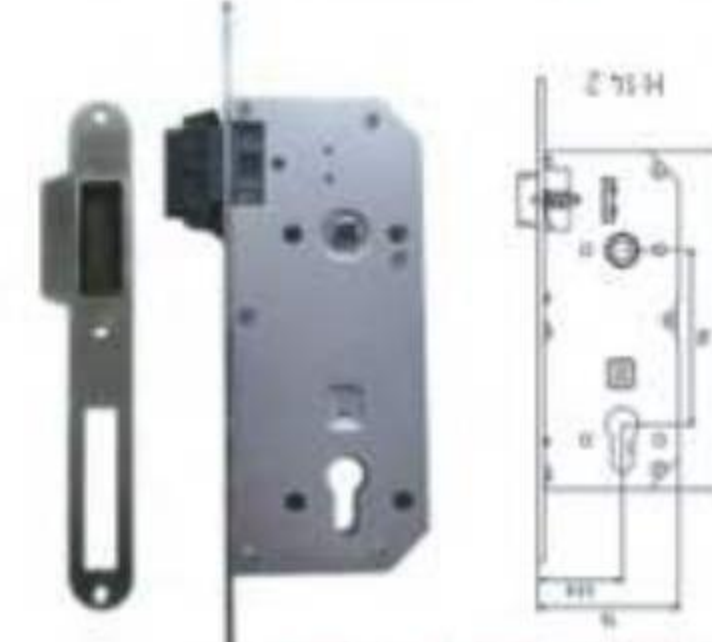
9045-CY MAGNET
